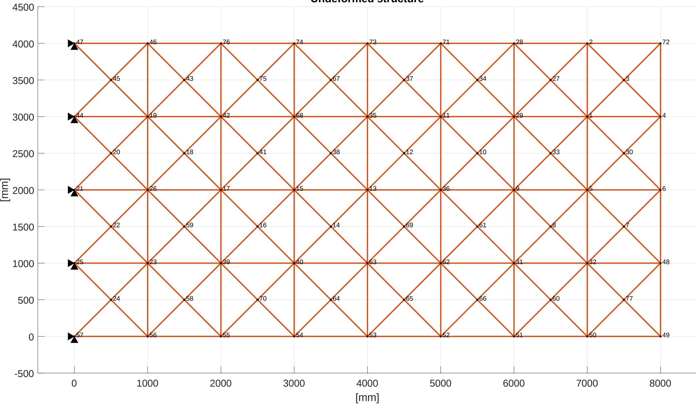
Undeformed structure
